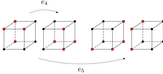
Figure 1.4: An illustration of R_5 , a strictly non-polar set of degree 2. Round points are feasible while square points are infeasible.
