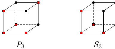
Figure 6.1: An illustration of P_3 and S_3 , the smallest non-cube-ideal sets. Round points are feasible while square points are infeasible.
