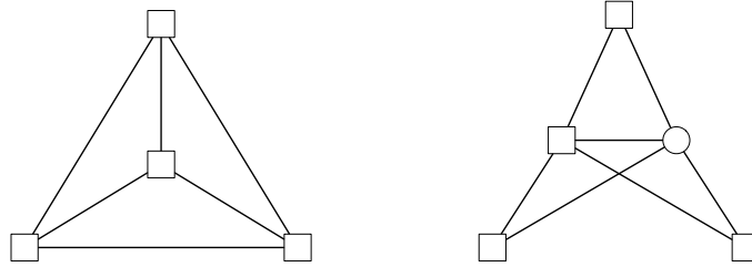
Figure 9.1: Left: plain quadrum, right: plain trifold. Square vertices are terminals.
