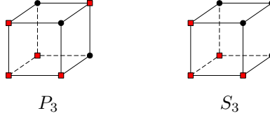
Figure 1.6: An illustration of P_3 and S_3 , the smallest non-cube-ideal sets.
