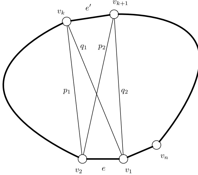
Figure 9.4: An illustration of graph G , where the edges in C are bold.
